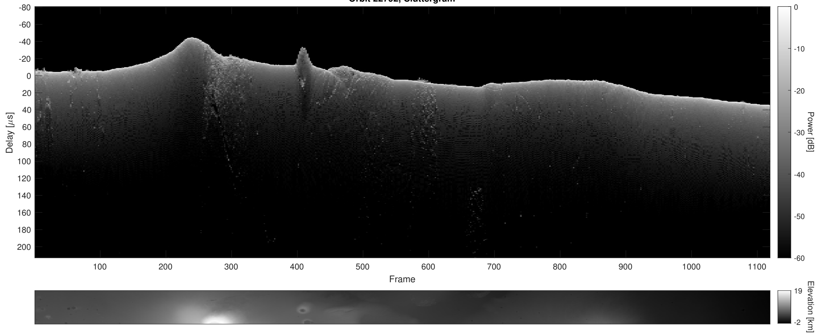
Orbit 22792, Cluttergram
