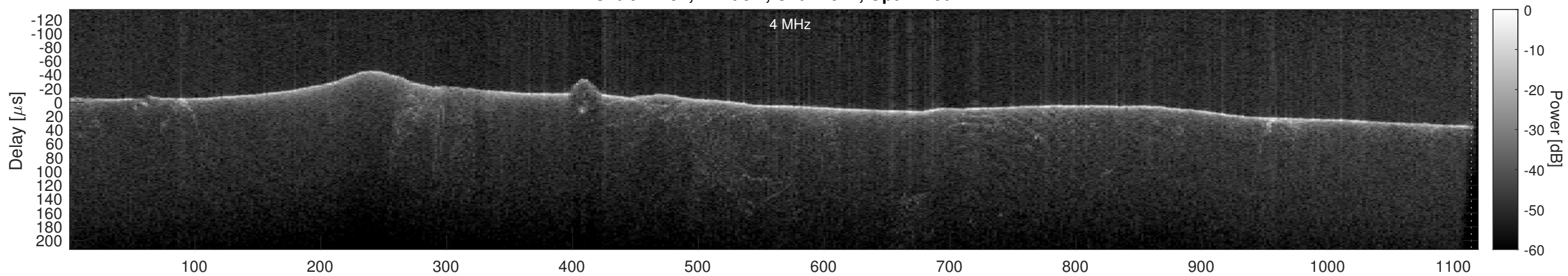
Orbit 22792, Cluttergram
