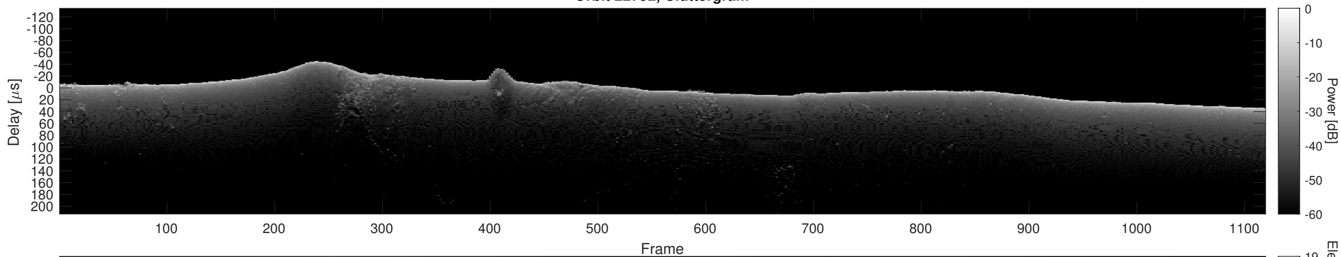
Orbit 22792, Cluttergram
