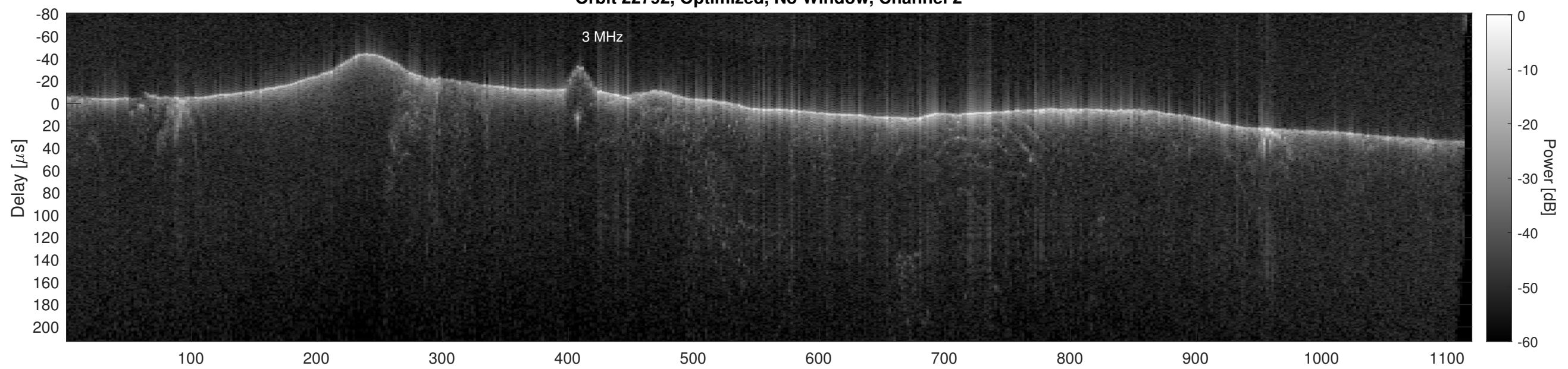
Orbit 22792, Cluttergram
