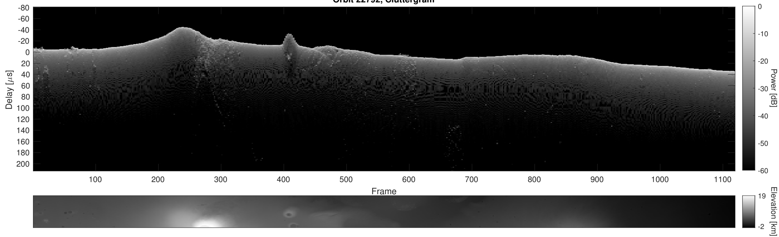
Orbit 22792, Cluttergram
