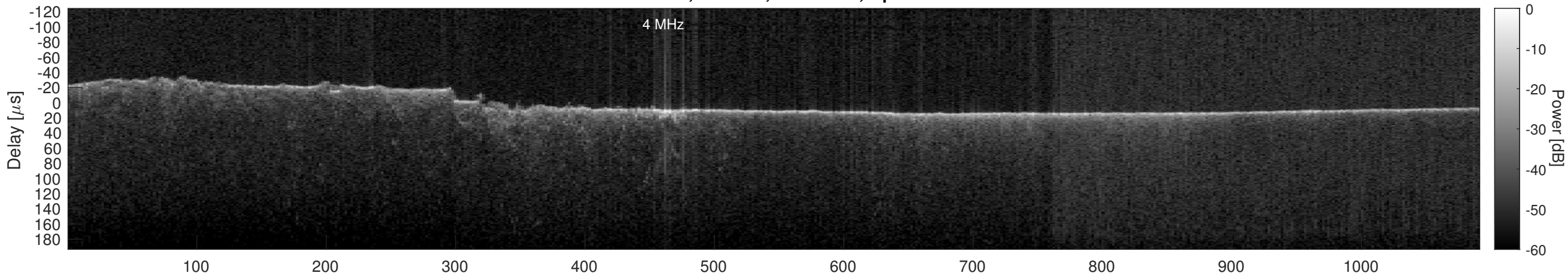
Orbit 22793, Cluttergram
