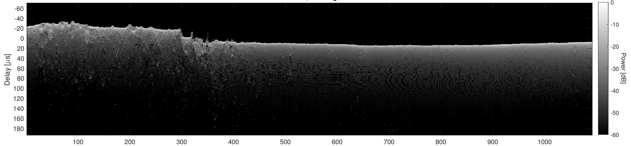
Orbit 22793, Cluttergram
