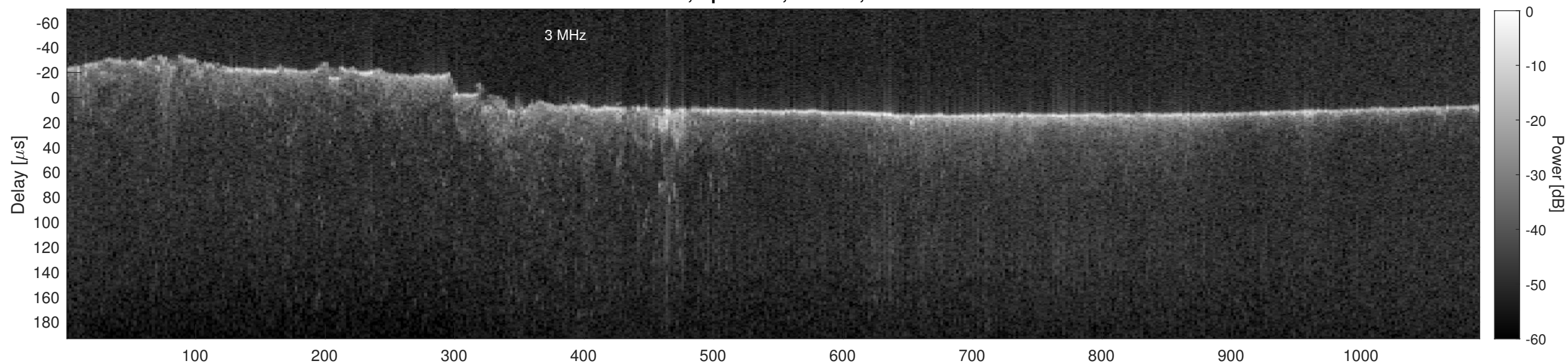
Orbit 22793, Cluttergram
