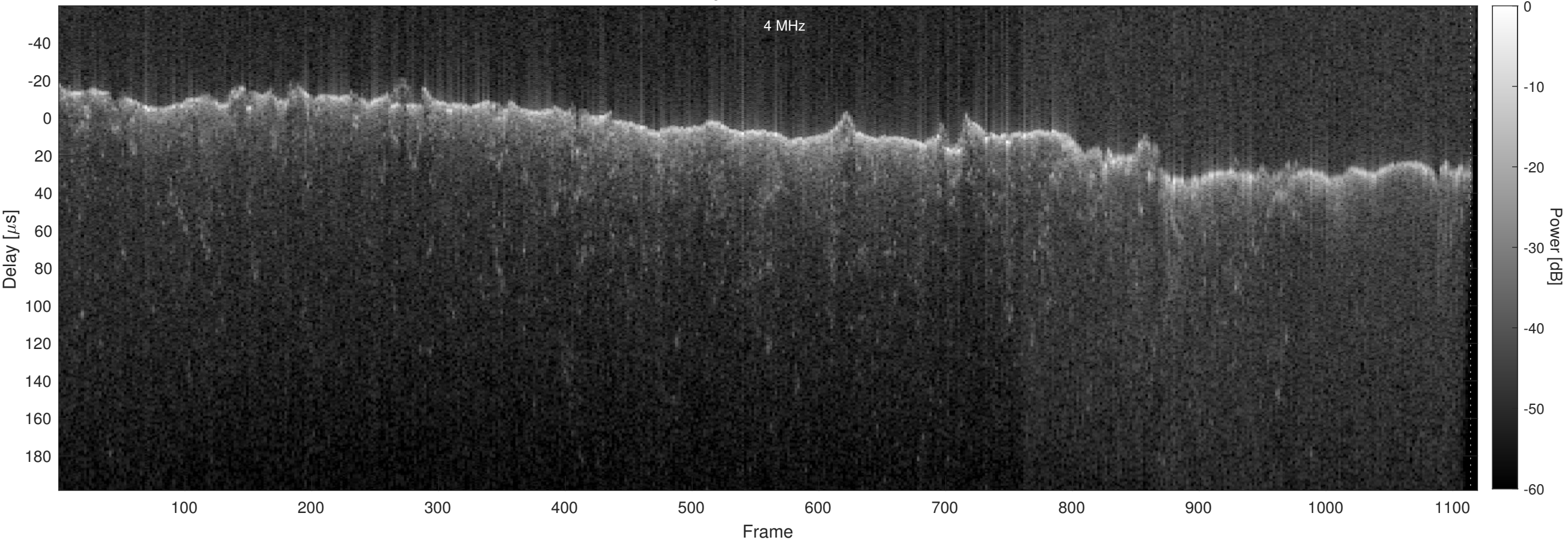
Orbit 22794, Chapman, No Window, Channel 2
