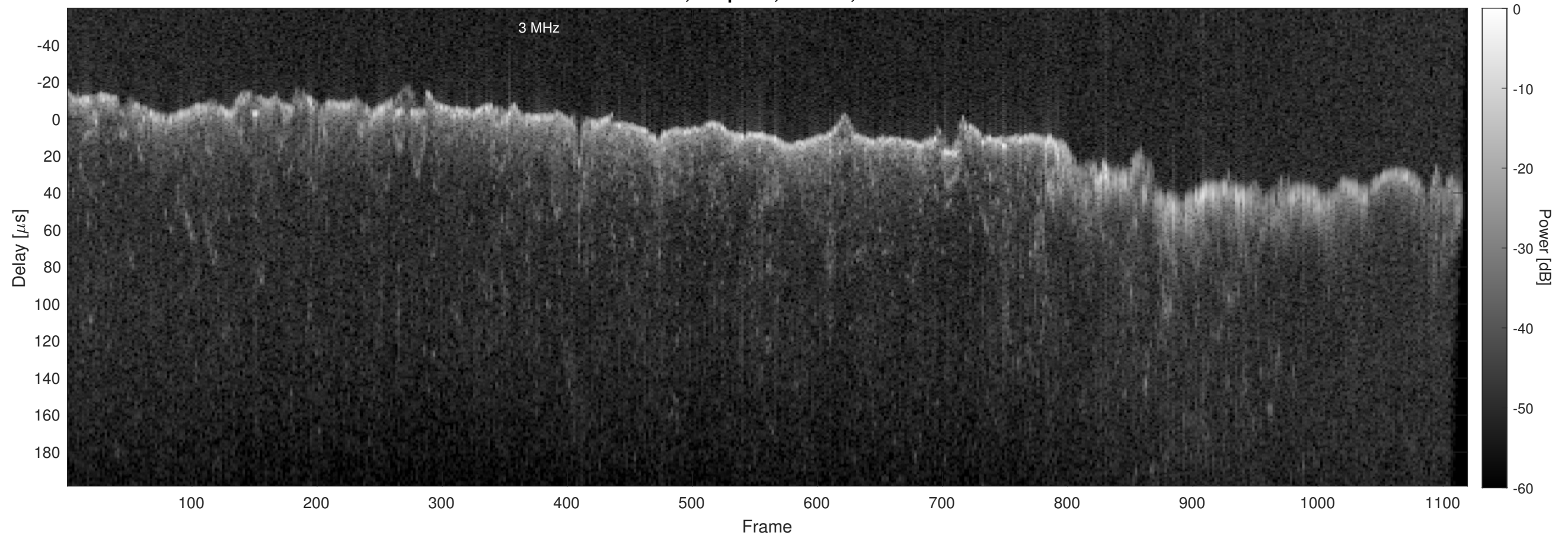
Orbit 22794, Chapman, Window, Channel 2
