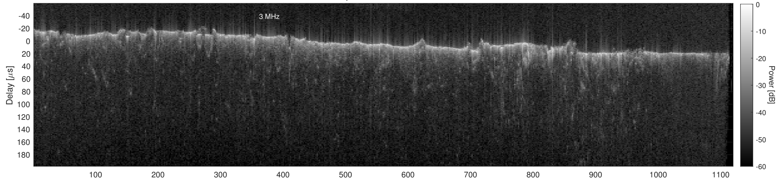
Orbit 22794, Cluttergram
