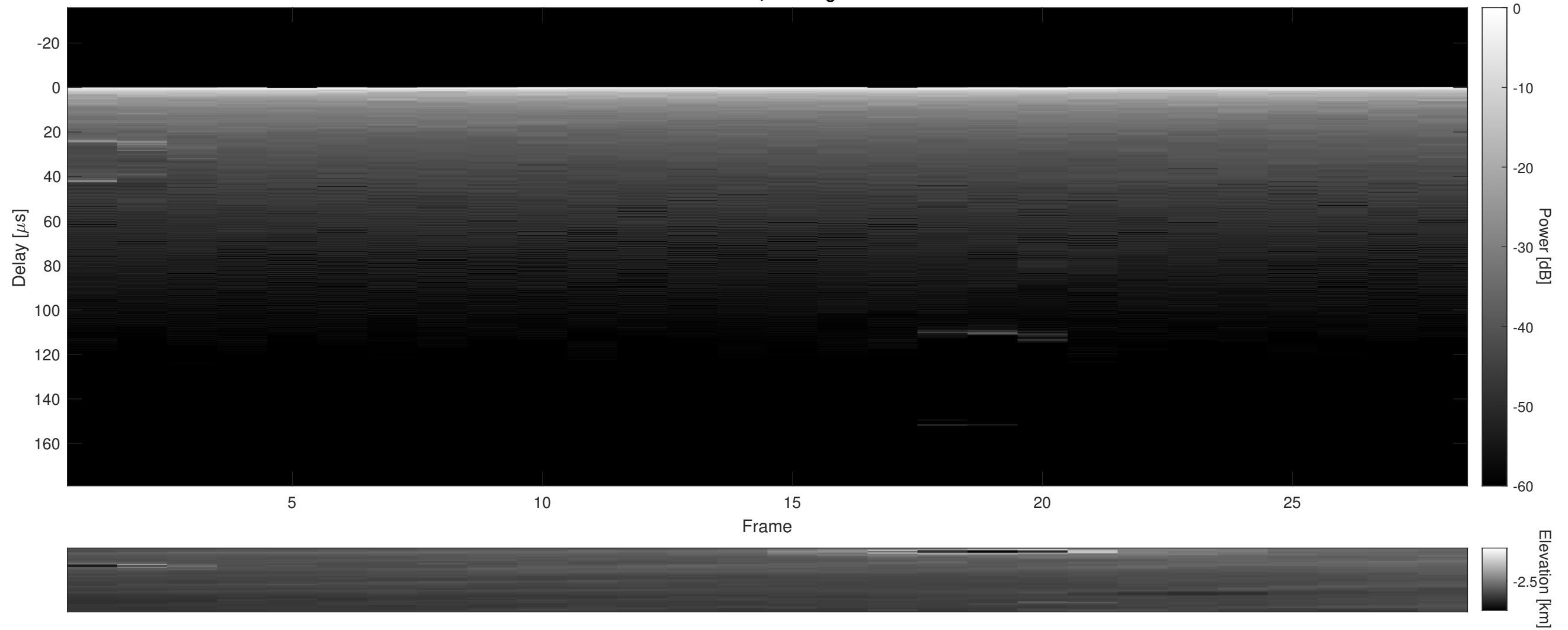
Orbit 22795, Cluttergram
