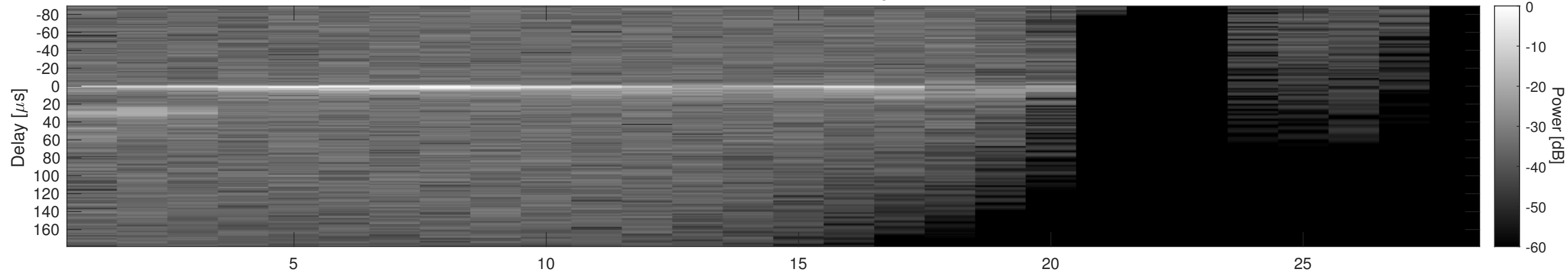
Orbit 22795, Cluttergram
