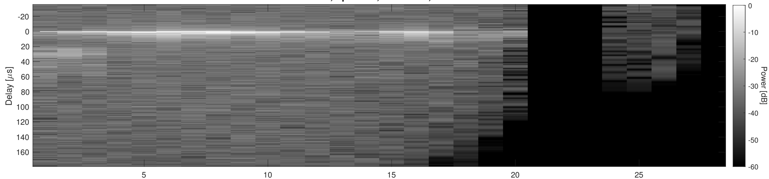
Orbit 22795, Cluttergram
