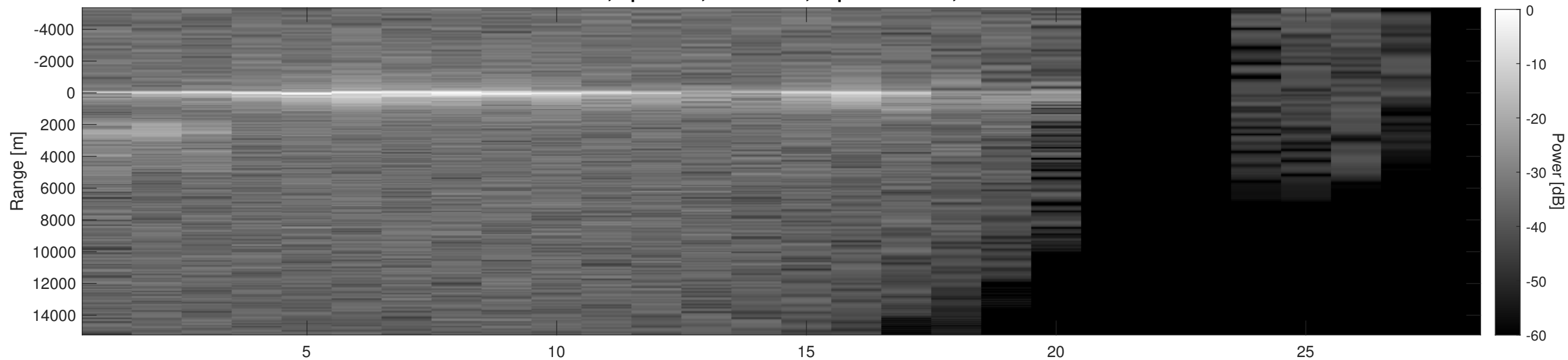
Orbit 22795, Depth-Corrected Cluttergram
