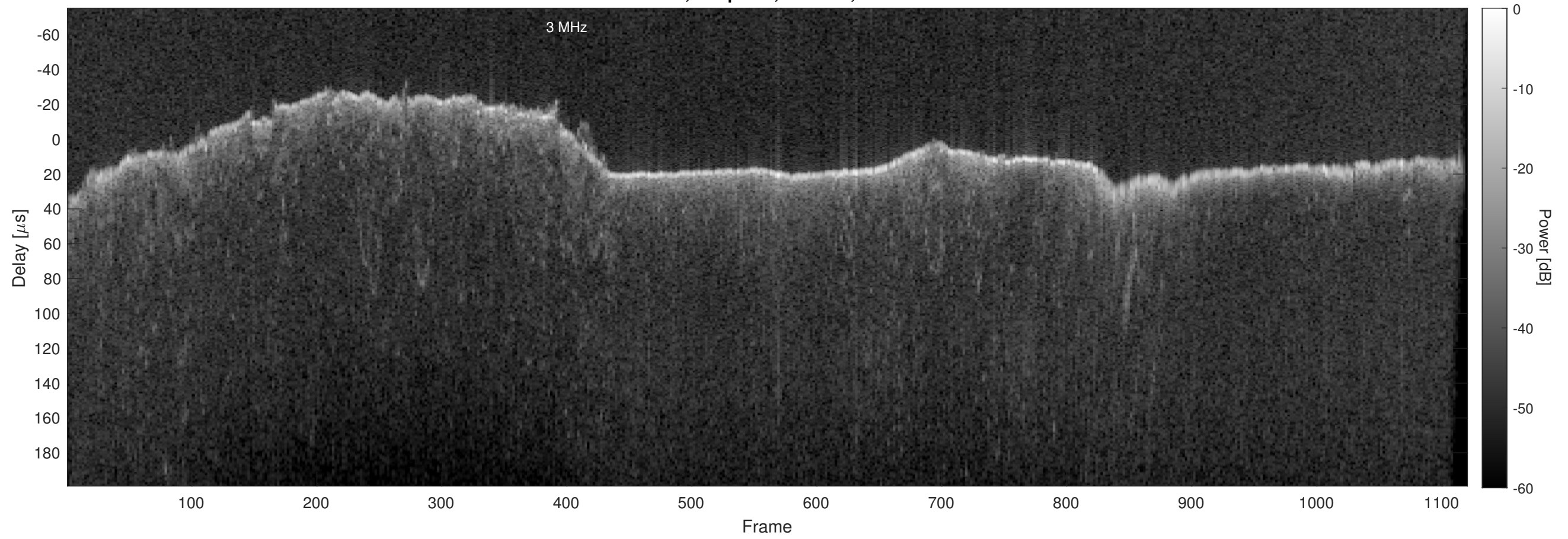
Orbit 22797, Chapman, Window, Channel 2
