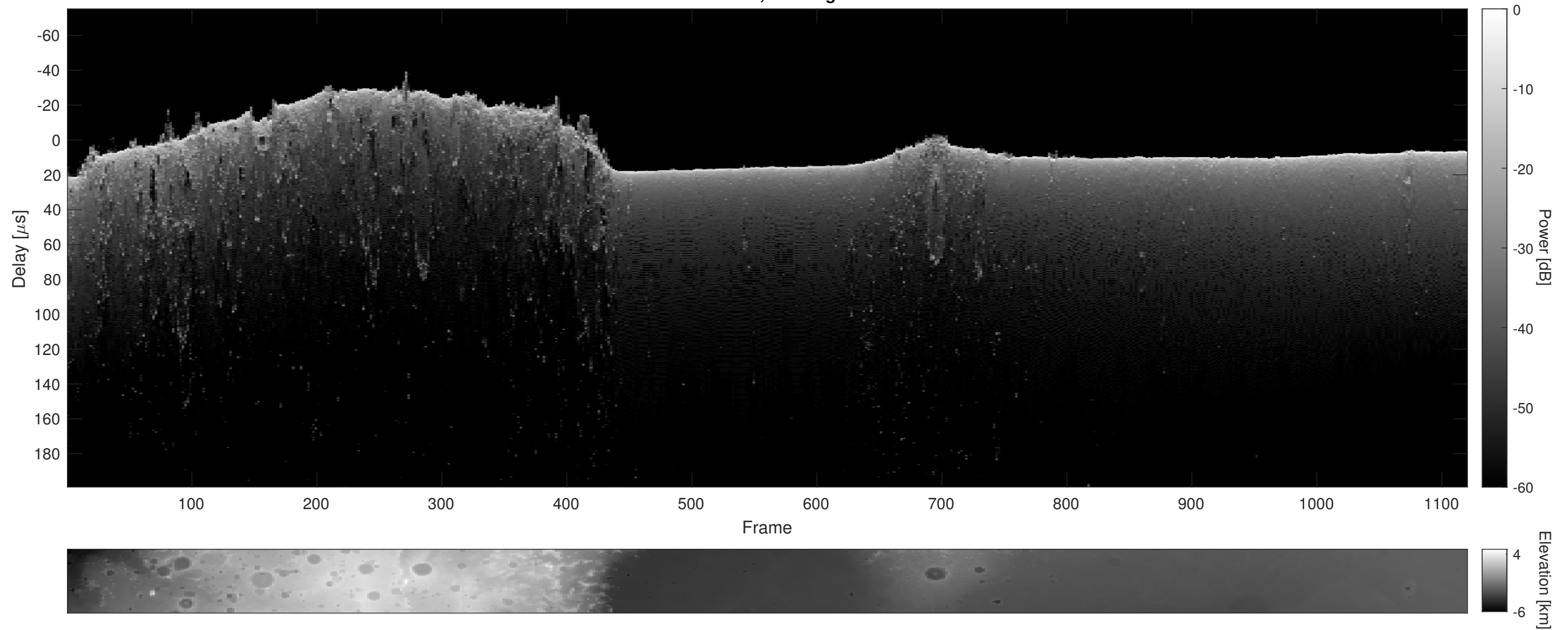
Orbit 22797, Cluttergram
