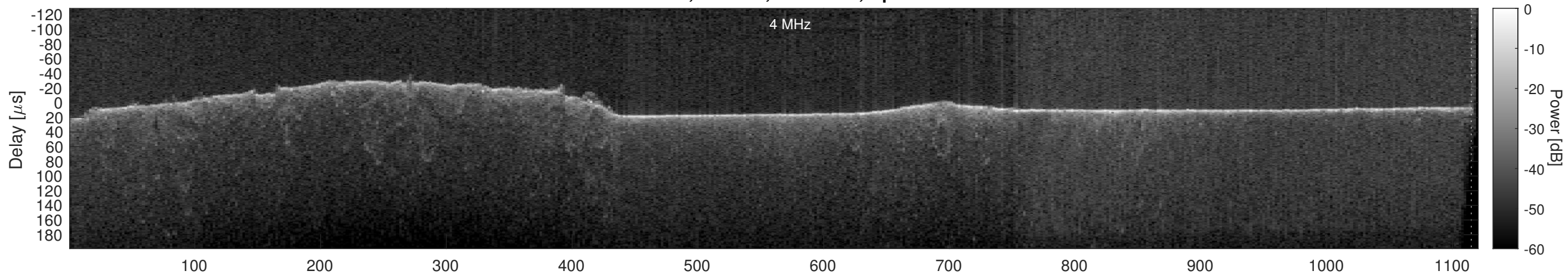
Orbit 22797, Cluttergram
