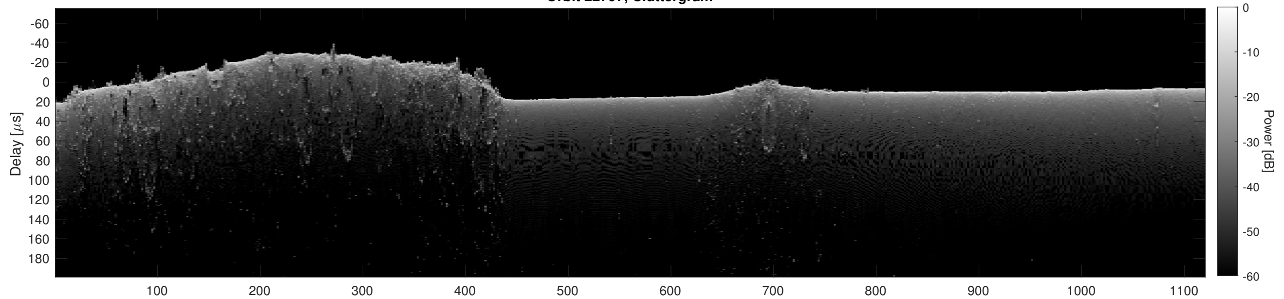
Orbit 22797, Cluttergram
