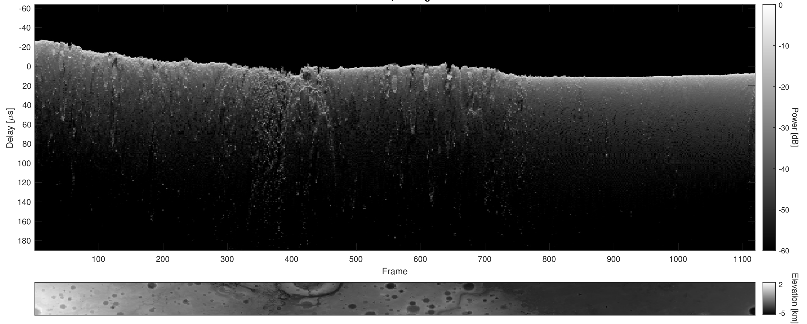
Orbit 22798, Cluttergram
