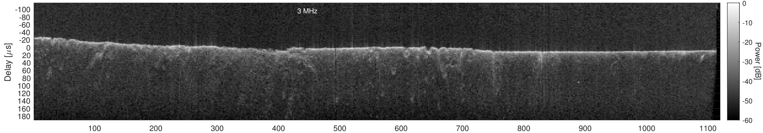
Orbit 22798, Cluttergram
