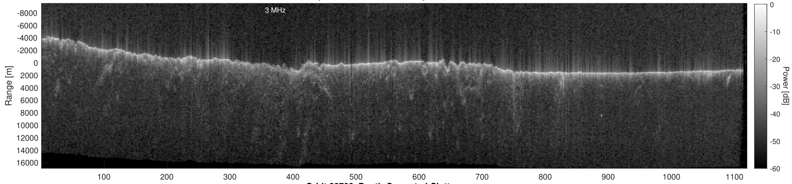
Orbit 22798, Depth-Corrected Cluttergram
