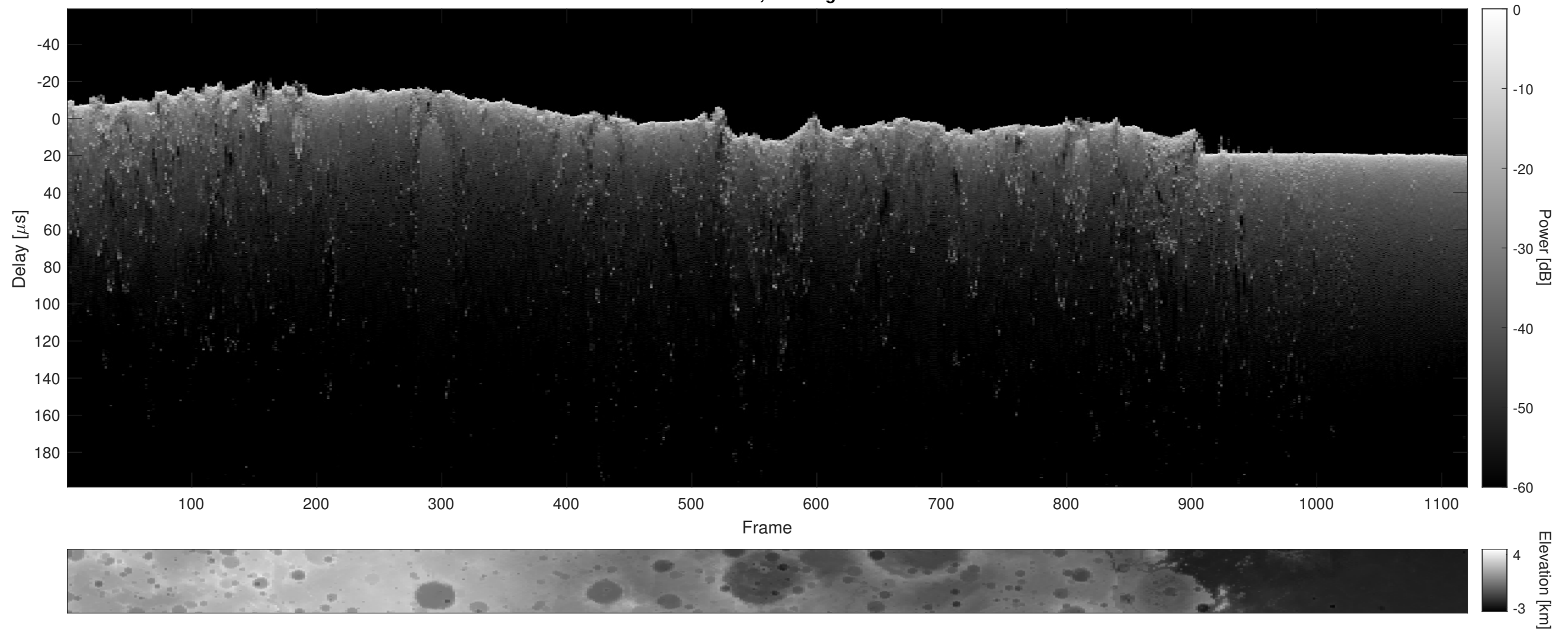
Orbit 22801, Cluttergram
