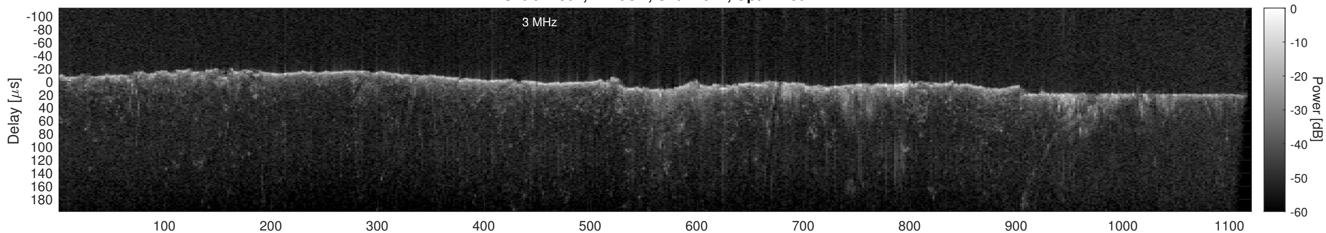
Orbit 22801, Cluttergram
