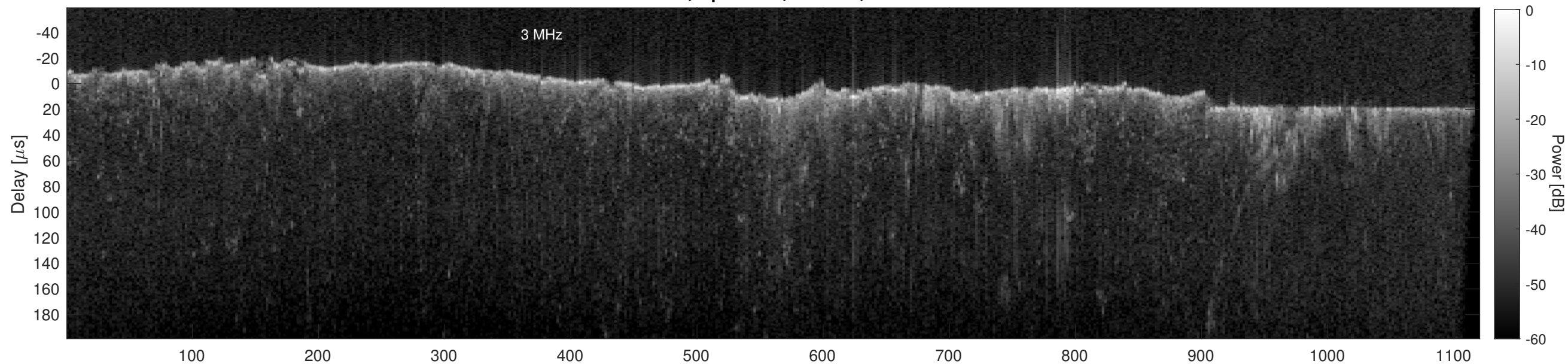
Orbit 22801, Cluttergram
