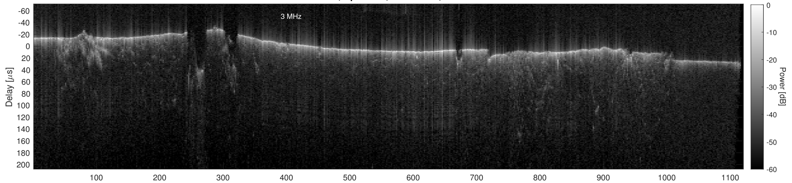
Orbit 22802, Cluttergram
