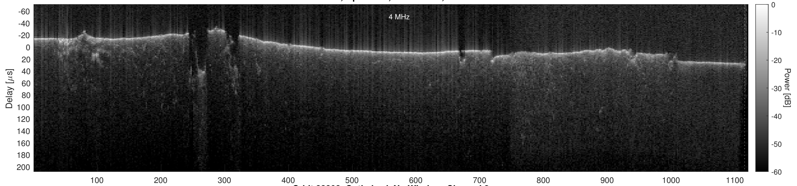
Orbit 22802, Optimized, No Window, Channel 2
