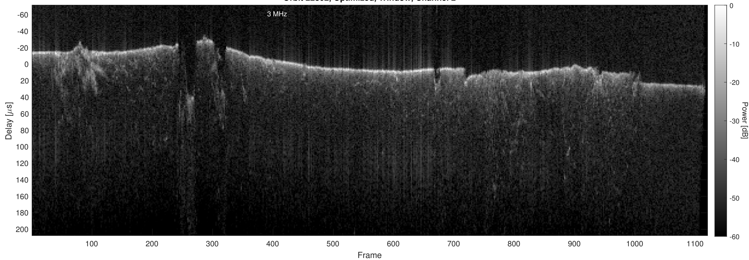
Orbit 22802, Optimized, Window, Channel 2
