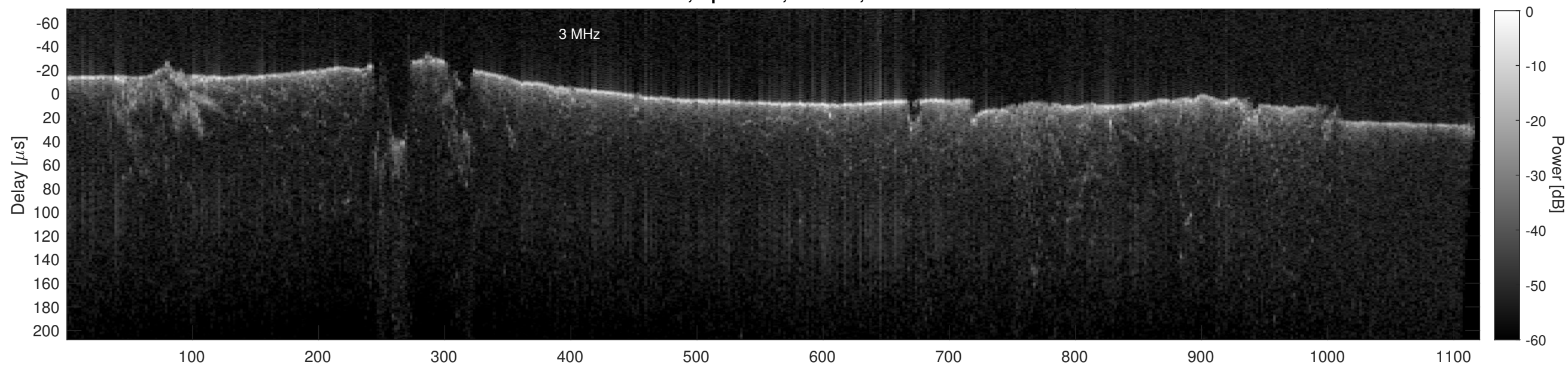
Orbit 22802, Cluttergram
