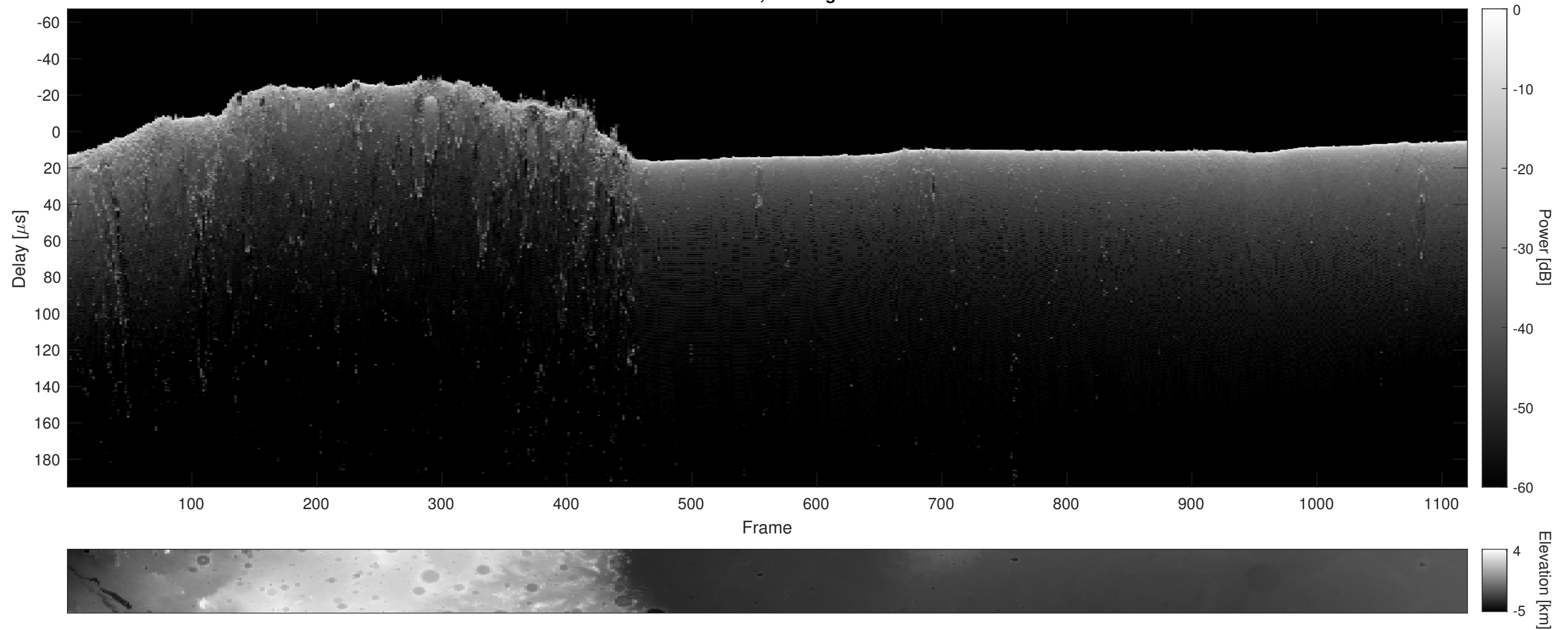
Orbit 22804, Cluttergram
