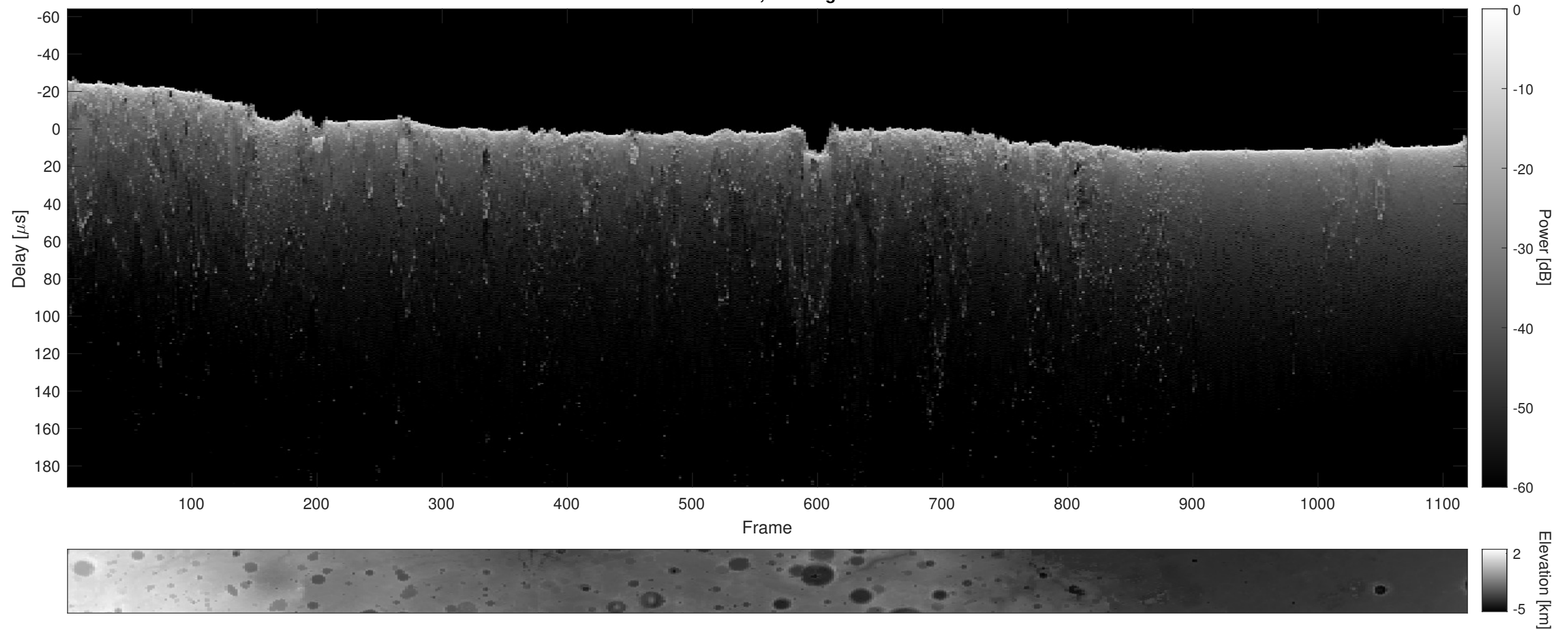
Orbit 22805, Cluttergram
