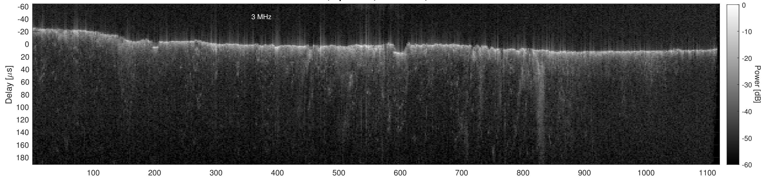
Orbit 22805, Cluttergram
