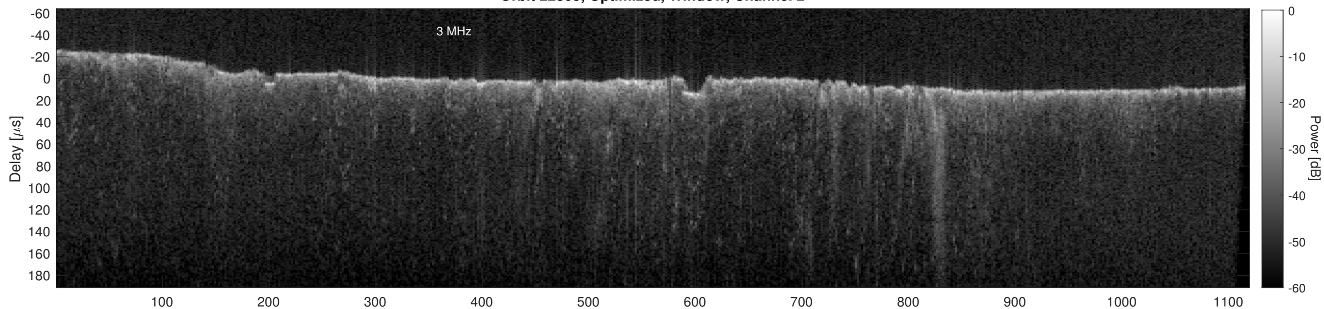
Orbit 22805, Cluttergram
