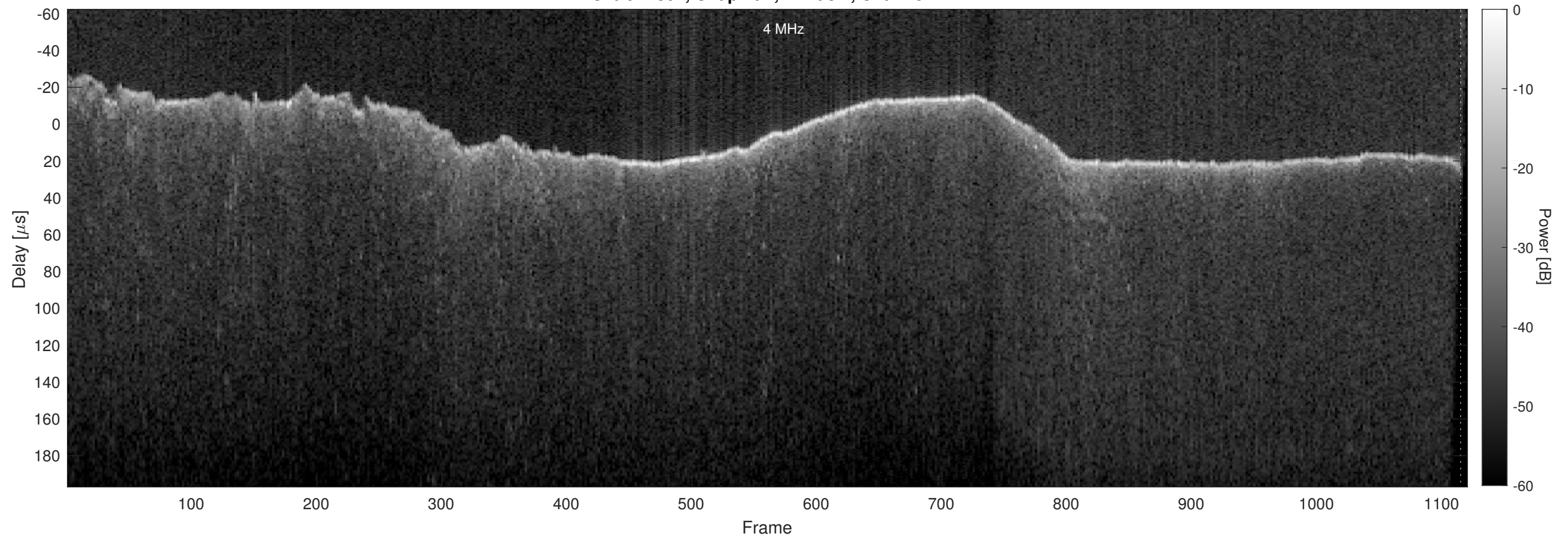
Orbit 22807, Chapman, Window, Channel 2
