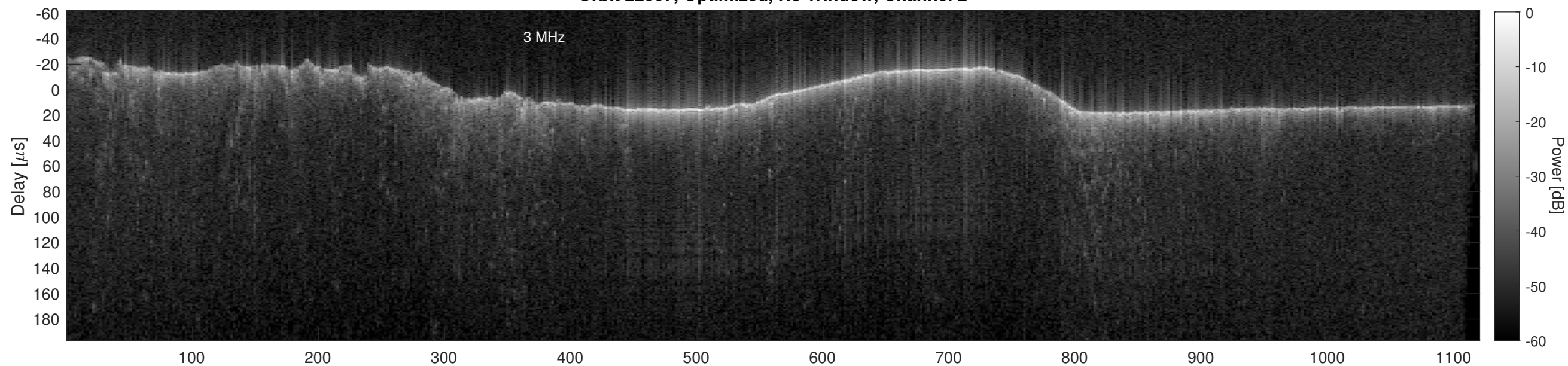
Orbit 22807, Cluttergram
