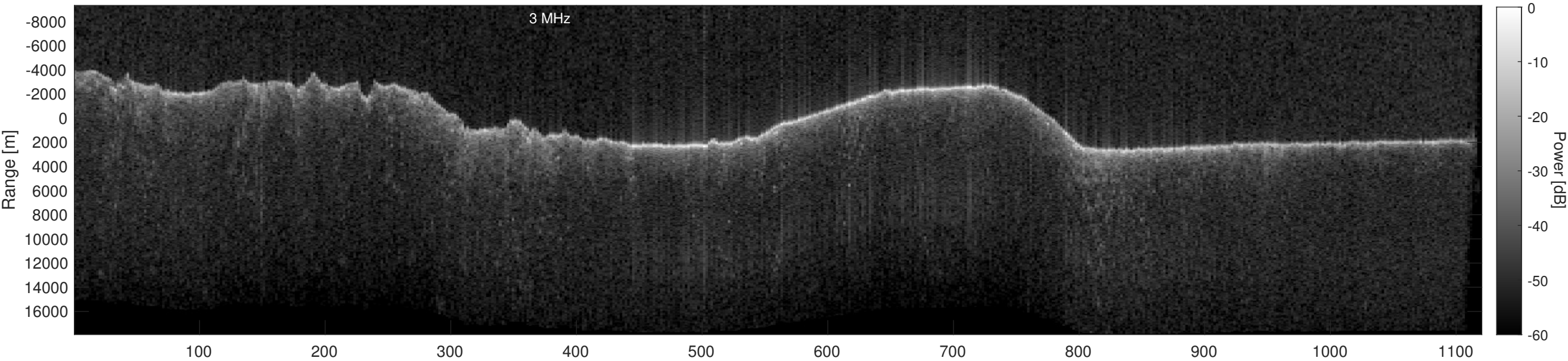
Orbit 22807, Depth-Corrected Cluttergram
