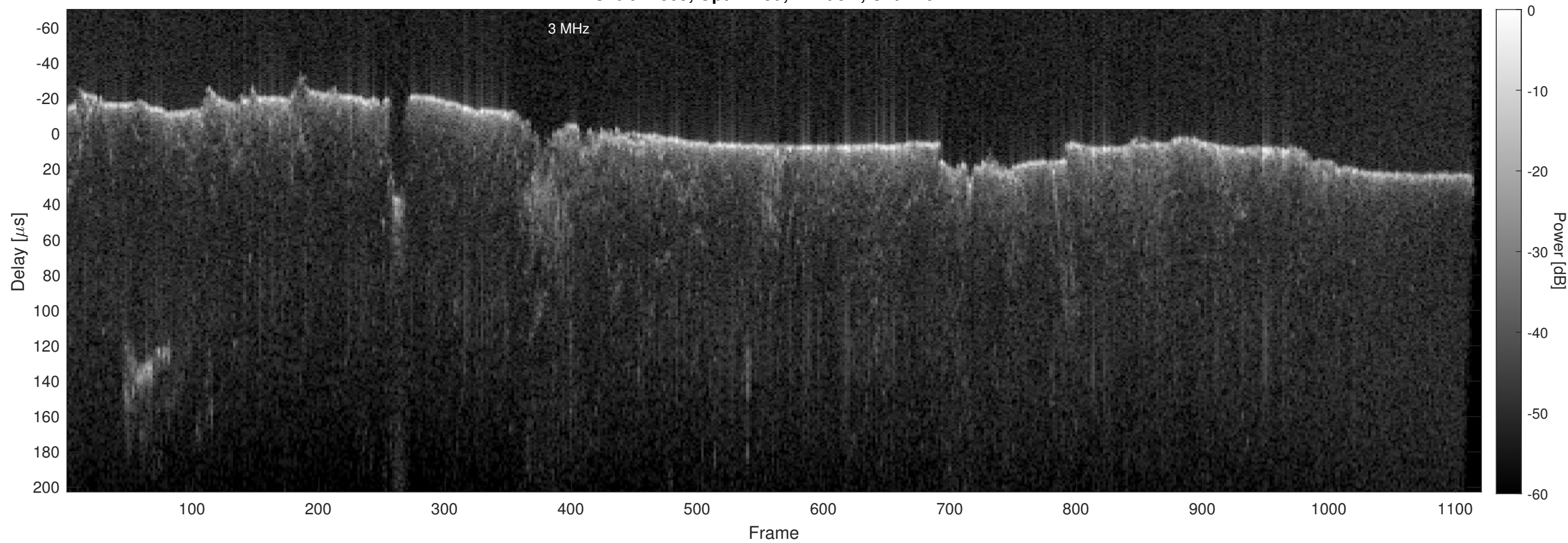
Orbit 22809, Optimized, Window, Channel 2
