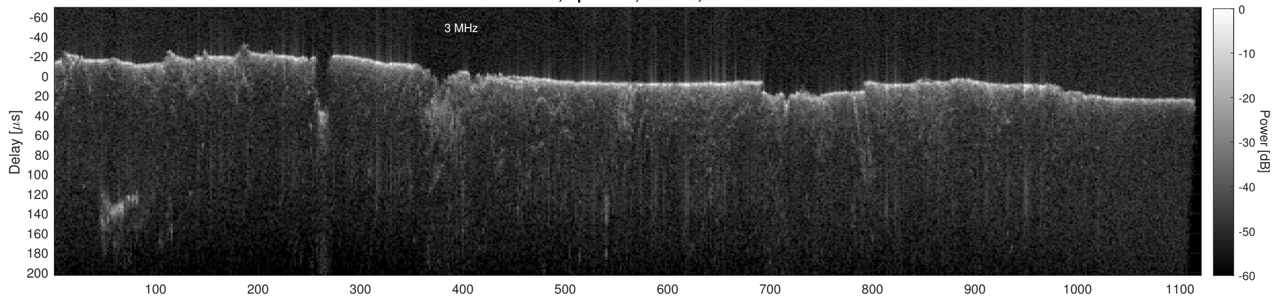
Orbit 22809, Cluttergram
