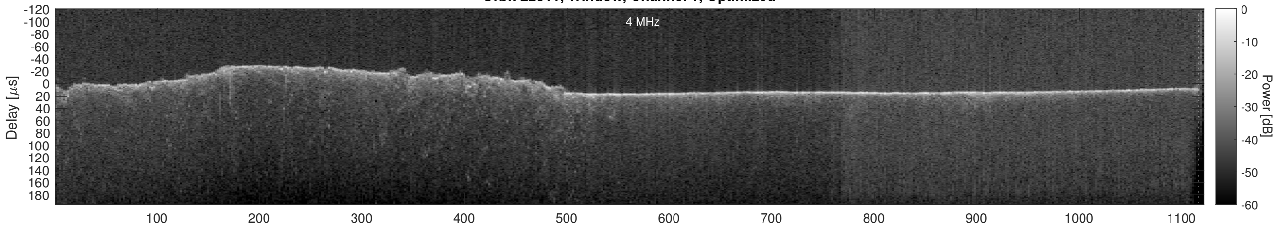
Orbit 22811, Cluttergram
