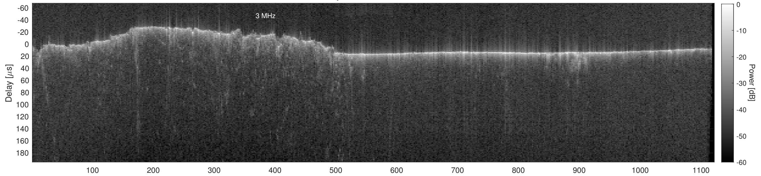
Orbit 22811, Cluttergram
