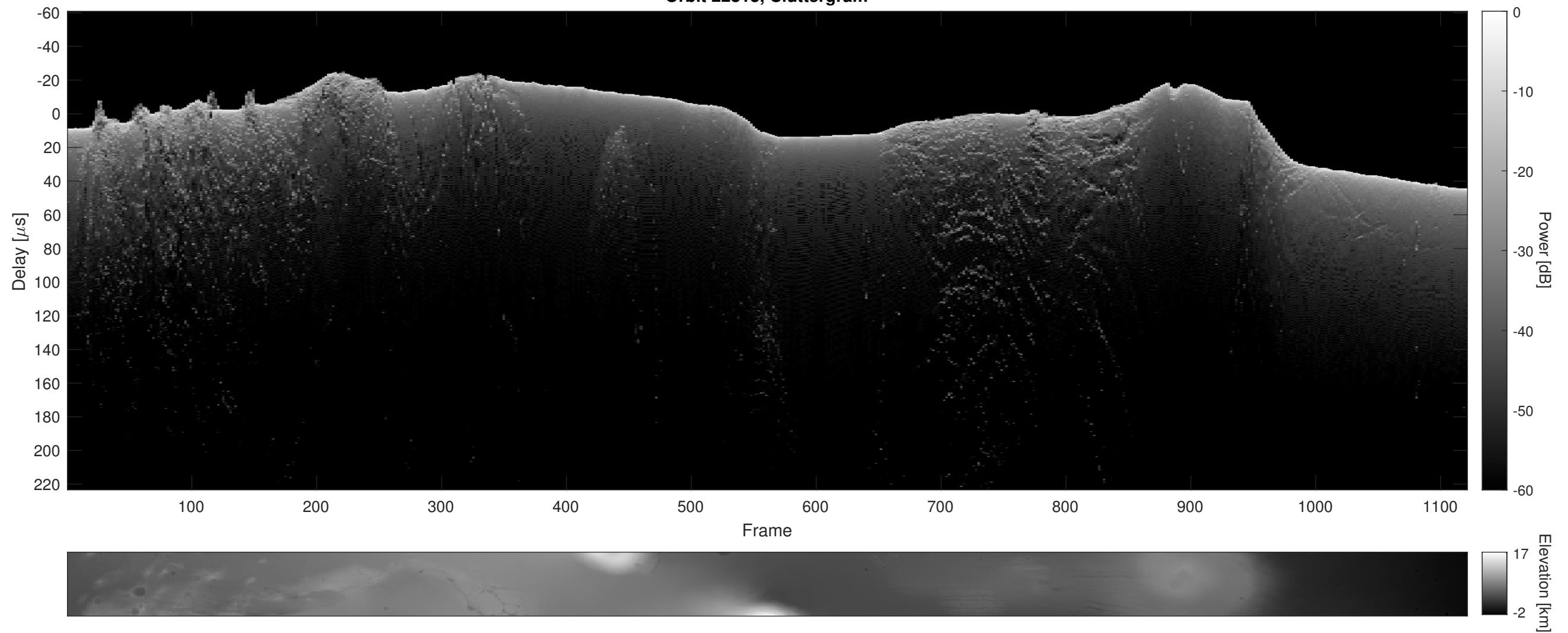
Orbit 22813, Cluttergram
