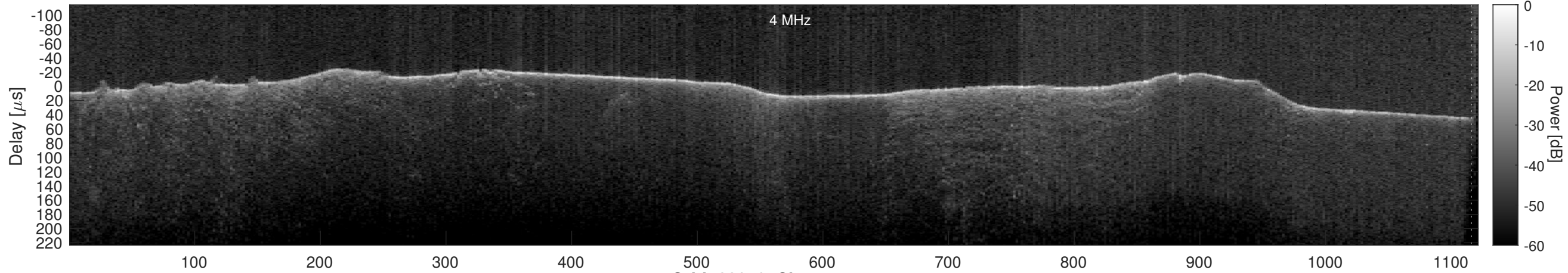
Orbit 22813, Cluttergram
