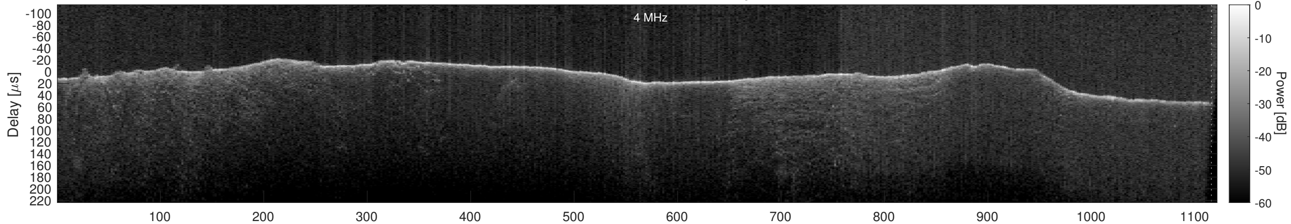
Orbit 22813, Window, Channel 1, Optimized
