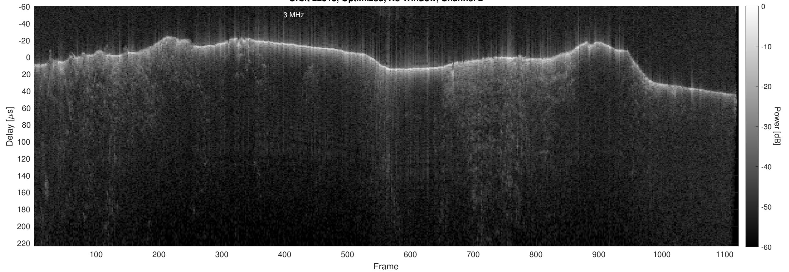
Orbit 22813, Optimized, No Window, Channel 2
