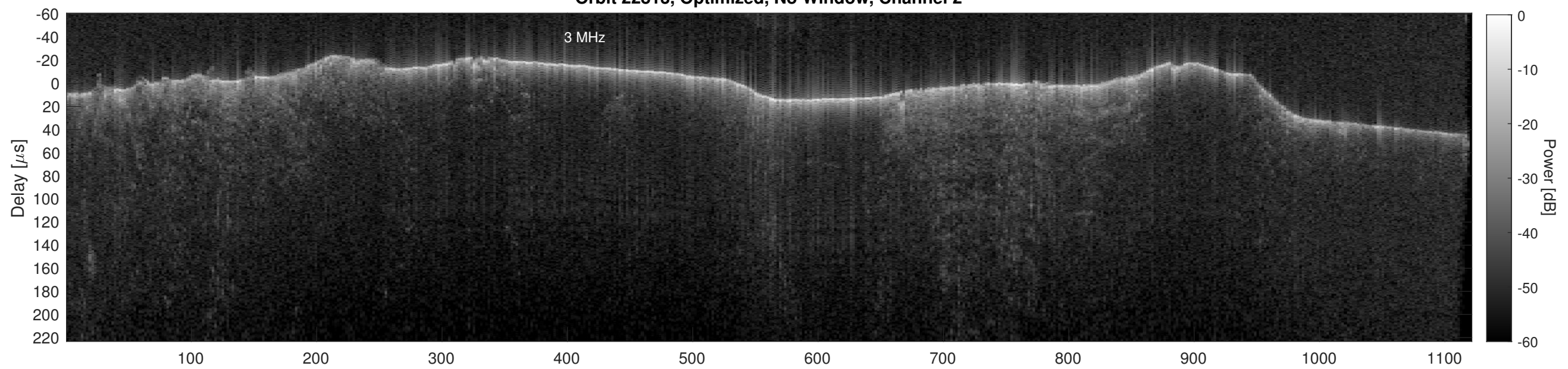
Orbit 22813, Cluttergram
