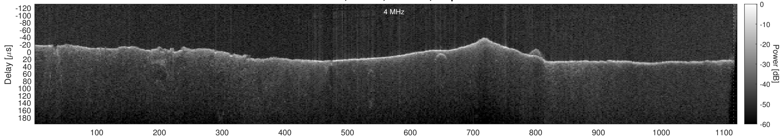
Orbit 22814, Window, Channel 1, Optimized
