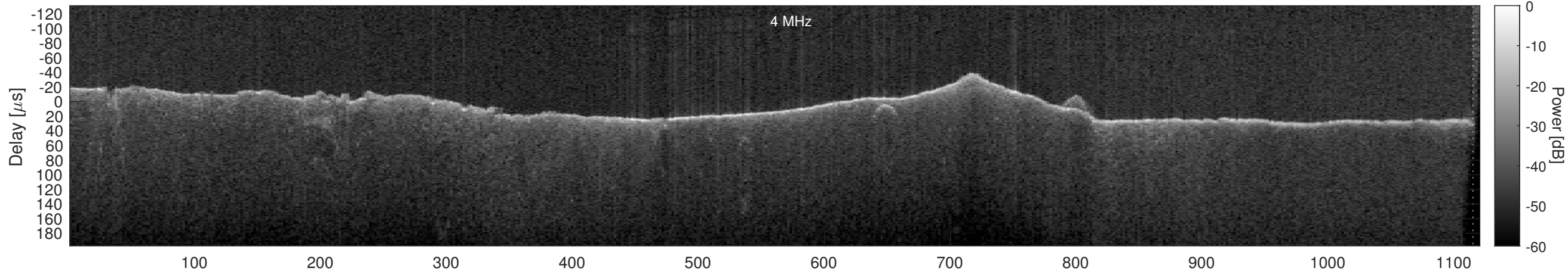
Orbit 22814, Window, Channel 1, Chapman
