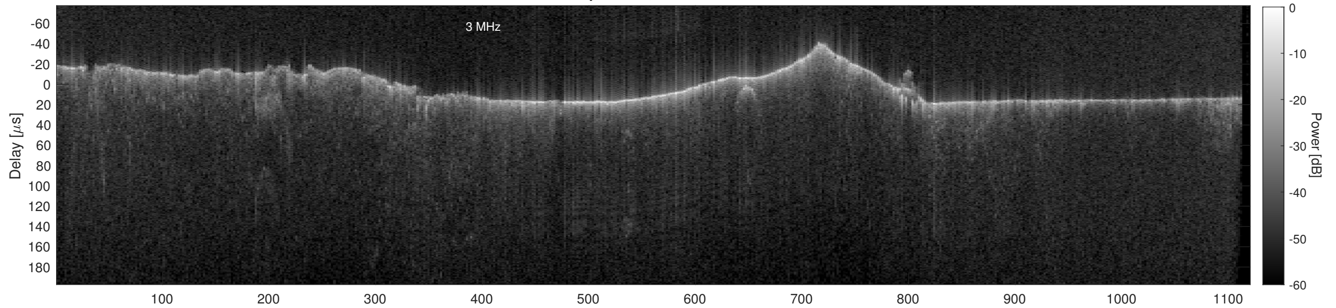
Orbit 22814, Cluttergram
