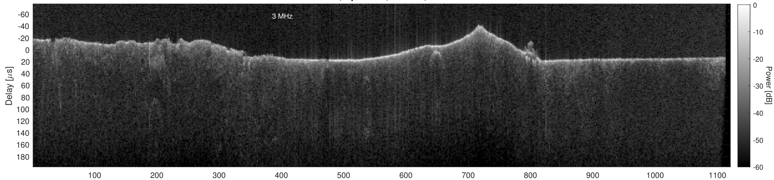
Orbit 22814, Cluttergram
