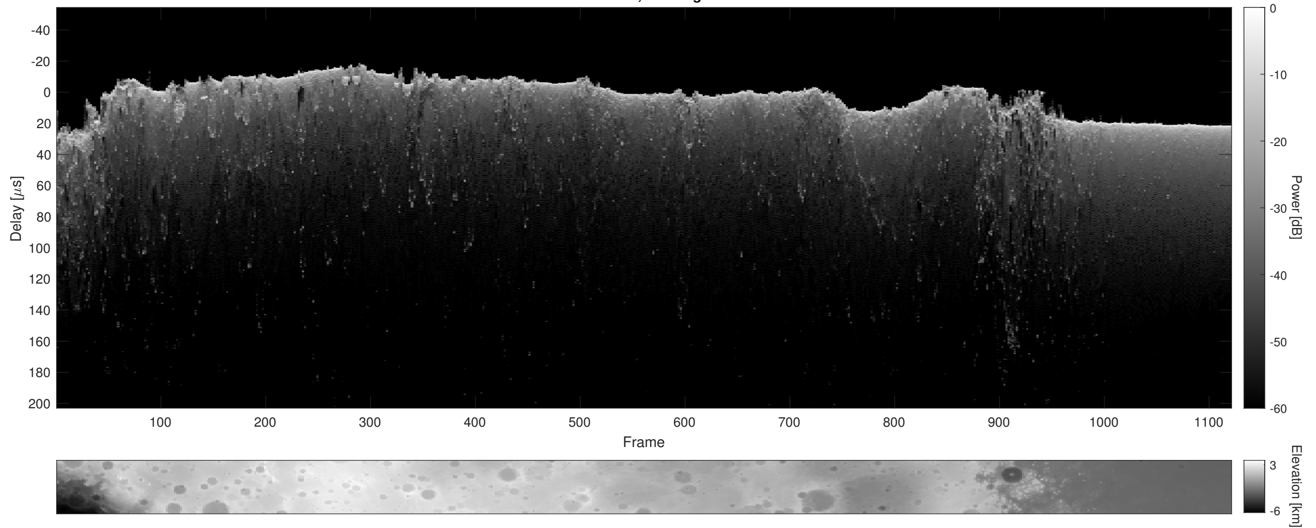
Orbit 22815, Cluttergram
