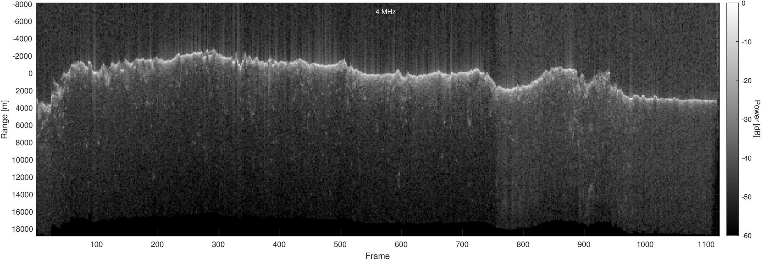
Orbit 22815, Optimized, No Window, Depth-Corrected, Channel 2
