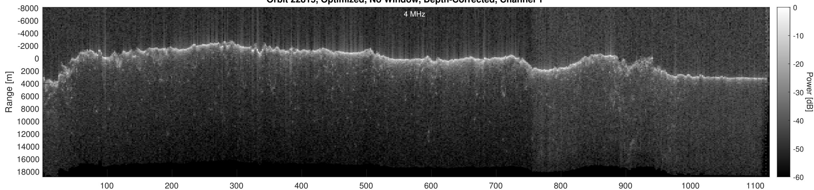
Orbit 22815, Optimized, No Window, Depth-Corrected, Channel 2
