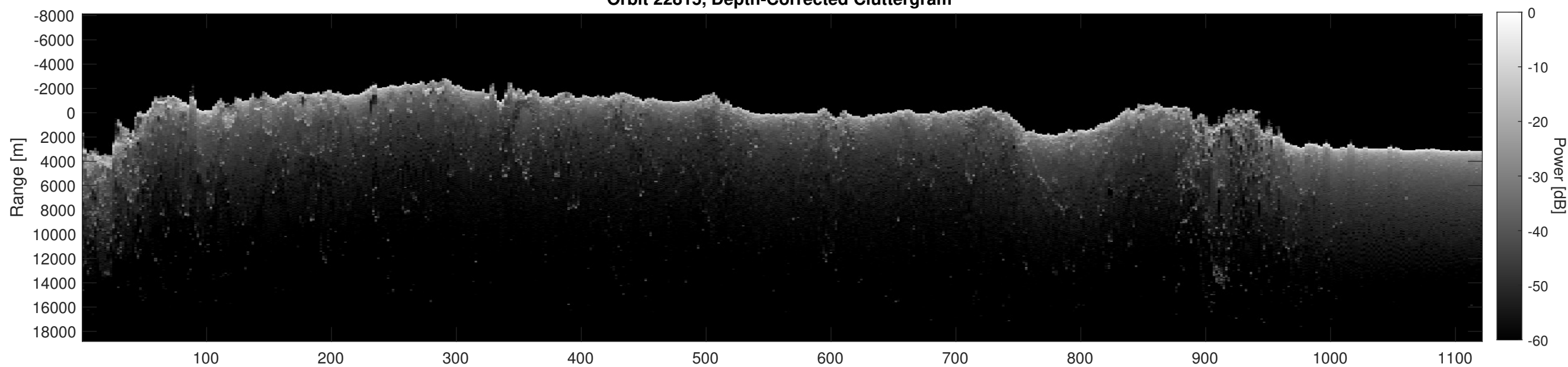
Orbit 22815, Depth-Corrected Cluttergram
