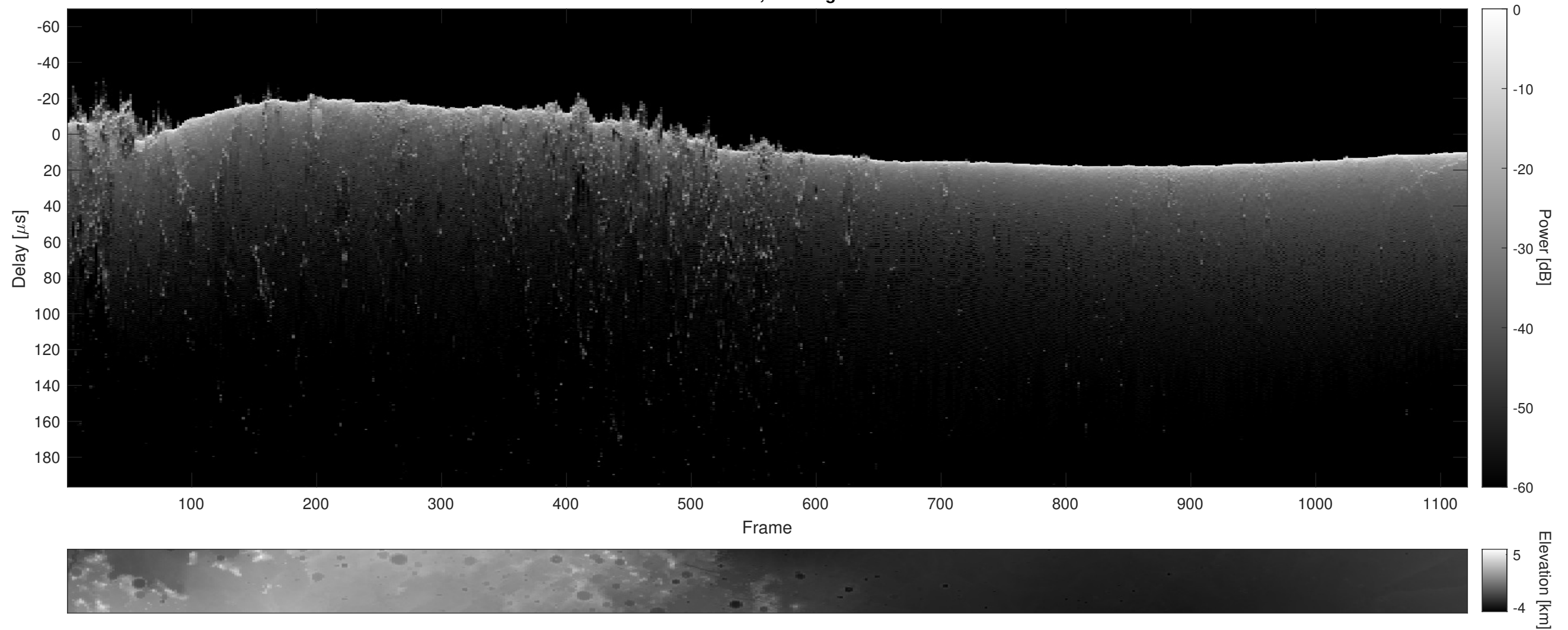
Orbit 22818, Cluttergram
